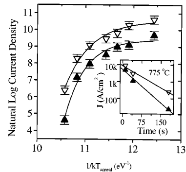
Fig. 3. Natural logarithm of current density versus the inverse of the annealing temperature ( T_{anneal} ) at constant biases and for 60 s anneals, where k_B is the Boltzmann factor. The open triangles represent the current at 350 mV, while the filled triangles represents the current at 25 mV after series resistance corrections. The data was fit to equations (4) and (5), giving an activation energy of 2.24 eV \pm 0.42 eV and 2.39 \pm 0.36 eV. The inset to Fig. 2 shows the decrease in current as a function of isothermal annealing time.
