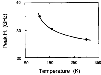
Fig. 2. Peak unity-current-gain cutoff frequency f_T (GHz) versus T (K) for a single 3.5 \times 10^{-6} - \mu\text{m}^2 emitter-finger HBT device.
