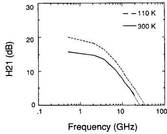
Fig. 1. H_{21} versus frequency for T = 300 K ( f_T = 26 GHz) and for 110 K ( f_T = 34 GHz).
