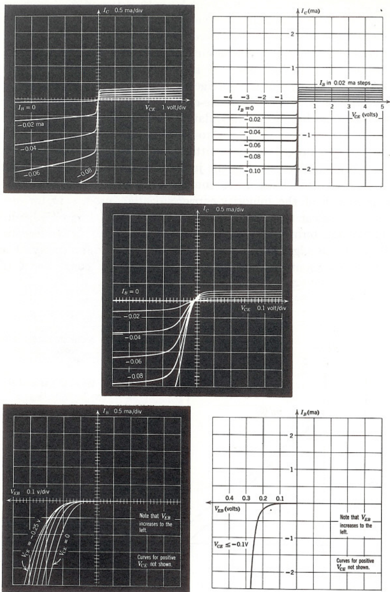
Fig. 9.7. Common-emitter transistor characteristics, showing the comparison between actual curves (left) and the predictions of the Ebers-Moll two-diode model (right).
