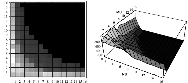
Fig. 20(e). Pentium III: Sensitivity of performance to M_U and N_U
