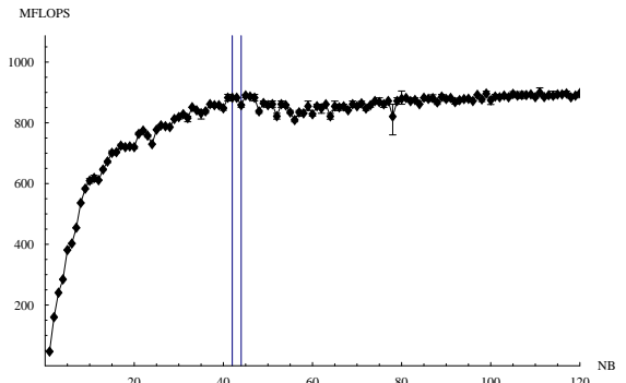
Fig. 20(g). Pentium III: Sensitivity of performance to N_B (zoomed)
