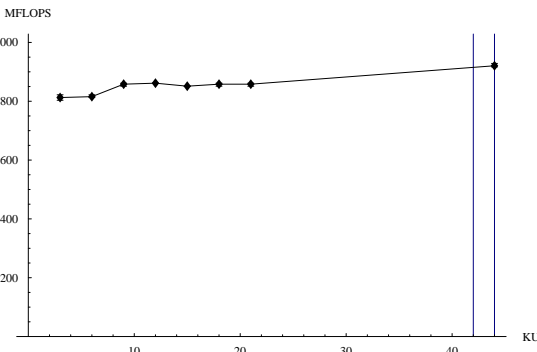
Fig. 20(h). Pentium III: Sensitivity of performance to K_U
