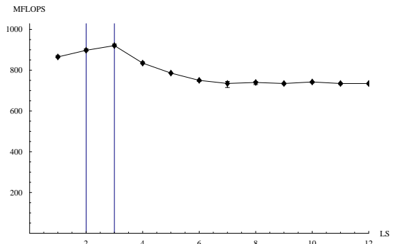
Fig. 20(i). Pentium III: Sensitivity of performance to L_s
