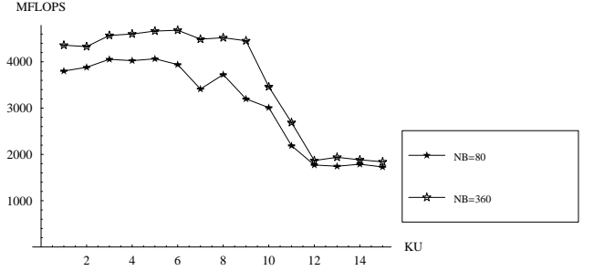
Fig. 6. Intel Itanium 2: Sensitivity of performance to K_U
