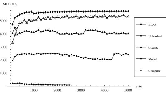
Fig. 17(d). Intel Itanium 2: MMM Performance
