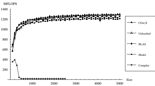
Fig. 13(d). IBM Power 3: MMM Performance
