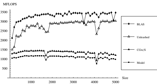
Fig. 21(d). Pentium 4: MMM Performance
